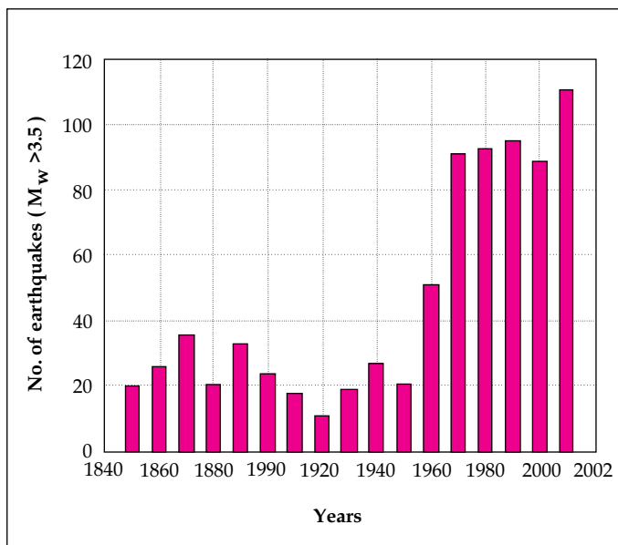
Figure 1. Past earthquake events in India in last 160 years
