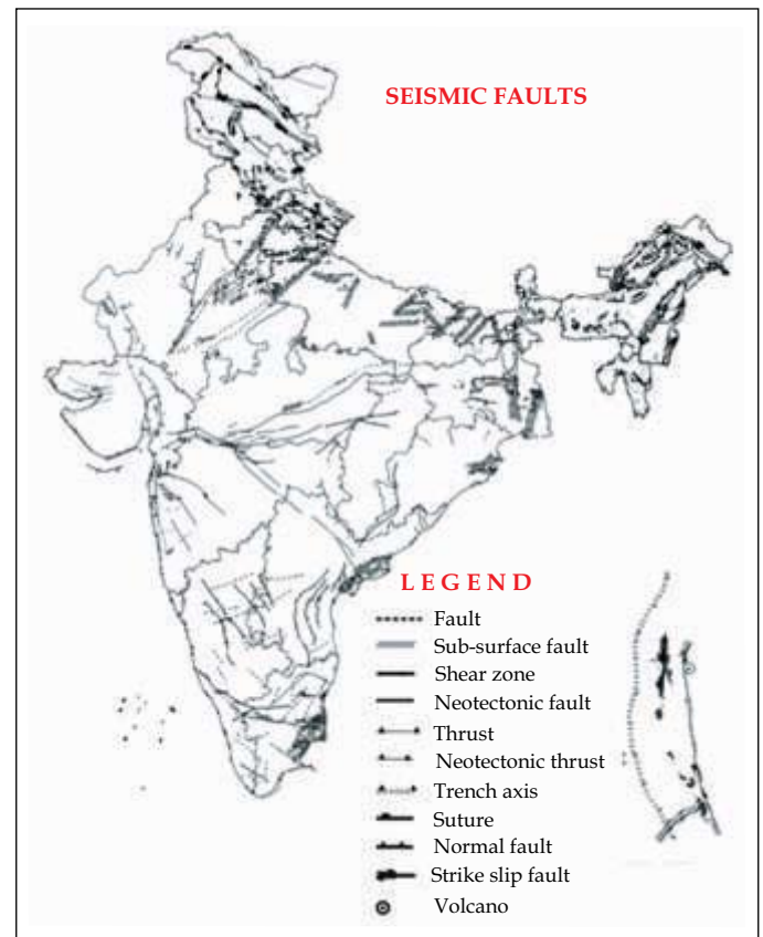
Figure 2. Map showing major faults in India (Based on GSI, 2003)
